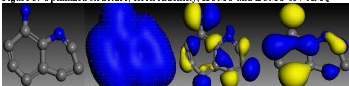
Figure 6: Optimized structure, electron density, HOMO and LUMO of 8-AMQ
