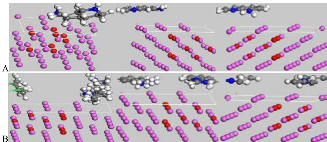
Figure 7: The final side snapshots of adsorbed 6-AMQ, 7-AMQ and 8-AMQ molecules.
