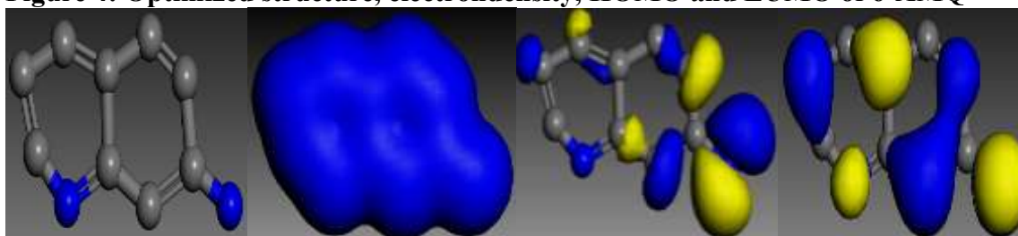
Figure 5: Optimized structure, electron density, HOMO and LUMO of 7-AMQ
